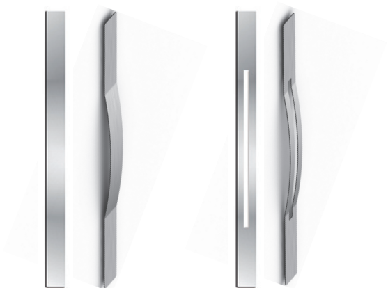
HQ (+opcja BIOKEY) HQ-ER (inox) - 100x5x1800 mm HQ-AL (aluminium) - 100x10x1800mm
